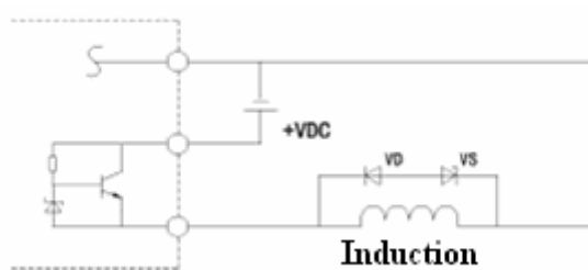
Figure 4-2-2 DC Transistor Output Regulated Diode Protection
