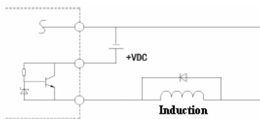
Figure 4-2-1 DC Transistor Output Normal Diode Protection
