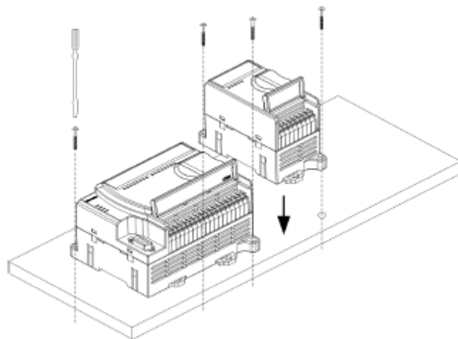
Figure 4-3-2 Panel Installation Mode
